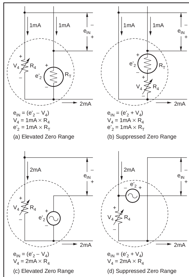
Figure 8. Elevation and Suppression Circuits
