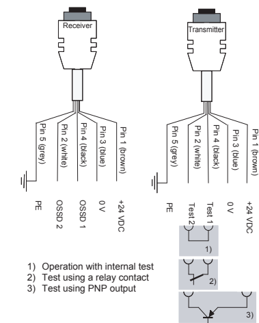
Figure 15: Wiring of the connecting cables of the M12/5 Pin connector
