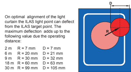
Figure 11: Adjustment with ILAS
