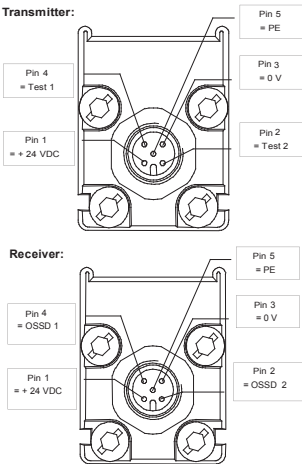
Figure 14: M12/5 Pin connector
