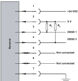
Figure 13: Terminal block connection (see also Figure 18)
